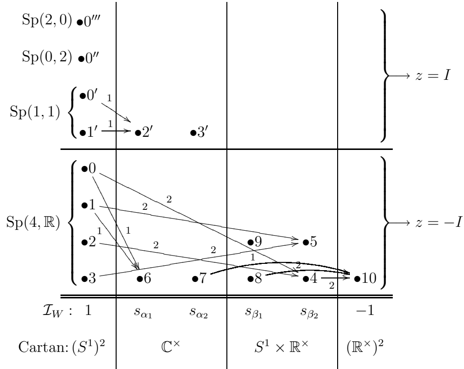
Figure 2: \mathcal{X} and Cayley transforms for \mathrm{Sp}(4)
