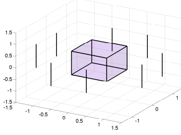
FIGURE 3. CS(SO(3, 2)_0, \delta_0) \times CS(SO(2, 1)_0, \delta_0)
