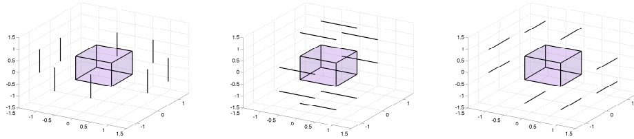
FIGURE 2. The three non-pseudospherical complementary series of Mp(6)
