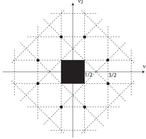
FIGURE 1. The spherical unitary dual of SO(3, 2)_0 .
